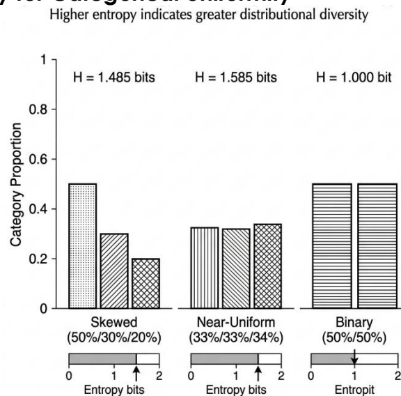
Figure 5: Shannon Entropy comparison across three representative categorical distributions. Skewed distributions (50/30/20) yield lower entropy (1.485 bits) indicating dominant class imbalance. Near-uniform distributions approach the theoretical maximum of \log_2(K) = \log_2(3) \approx 1.585 bits. Binary balanced distributions produce exactly 1.000 bit, the fundamental unit of binary information. PyDataQuality reports entropy as a column statistic, enabling detection of degenerate features (entropy \approx 0 ) indicating near-constant columns.
