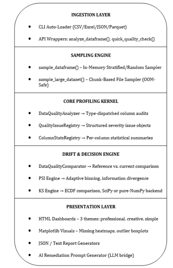
Figure 2: PyDataQuality Architecture Stack. System architecture diagram illustrating the 5-layer decoupled design of PyDataQuality. Data flows from ingestion through an O(1) -capped sampling engine, into a core profiling kernel, optionally through a drift & decision engine, and finally to the presentation layer for dashboarding and AI remediation generation.
